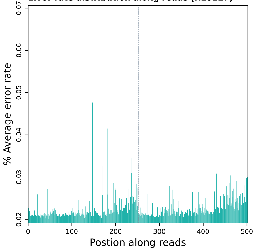
Error rate distribution along reads (R10127)
